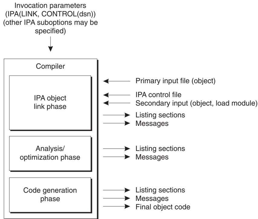
Figure 109. IPA Link step processing
