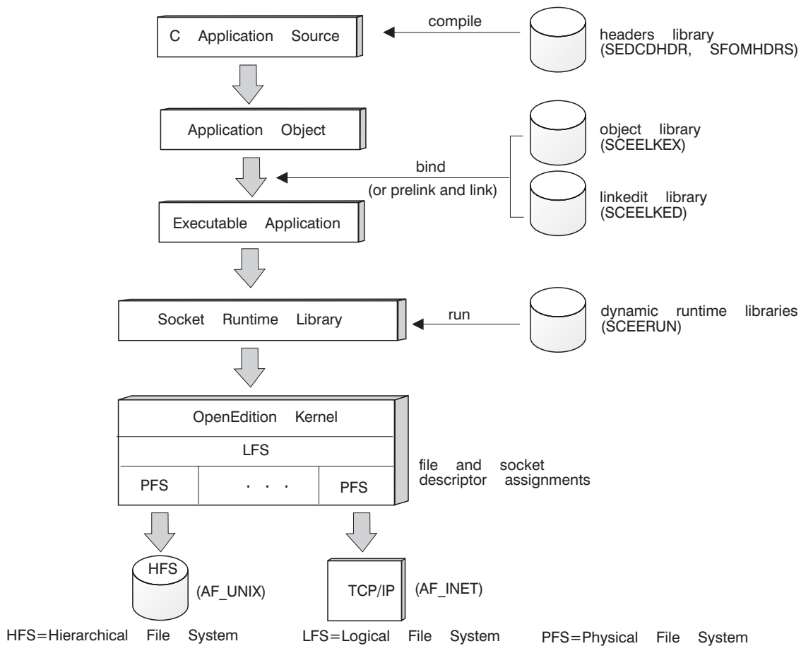
Figure 124. A Conceptual Overview of the Compile, Bind, and Run Steps
