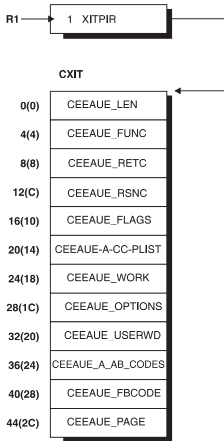
Figure 160. Interface for Assembler User Exits
