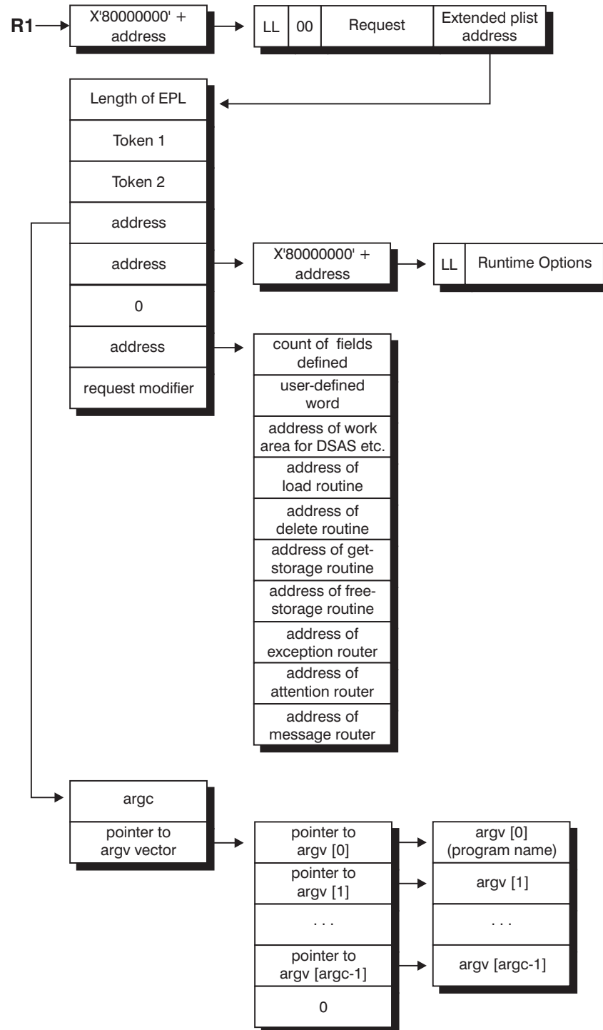
Figure 44. Interface for Preinitializable Programs
