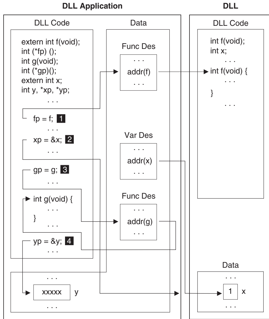
Figure 57. Pointer Assignment in DLL code
