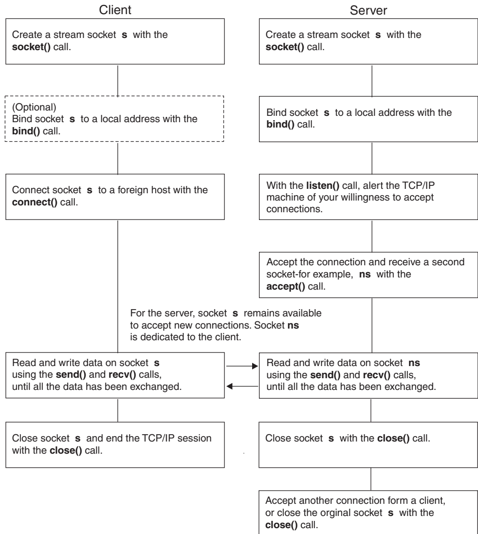
Figure 111. A Typical Stream Socket Session
