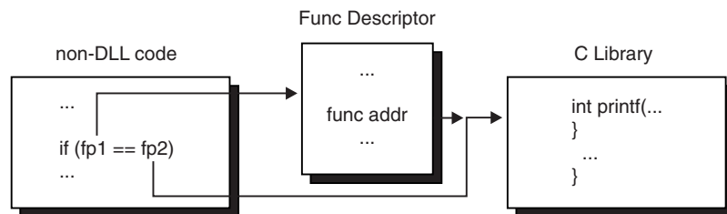
Figure 71. Comparison of Function Pointers in non-DLL code
