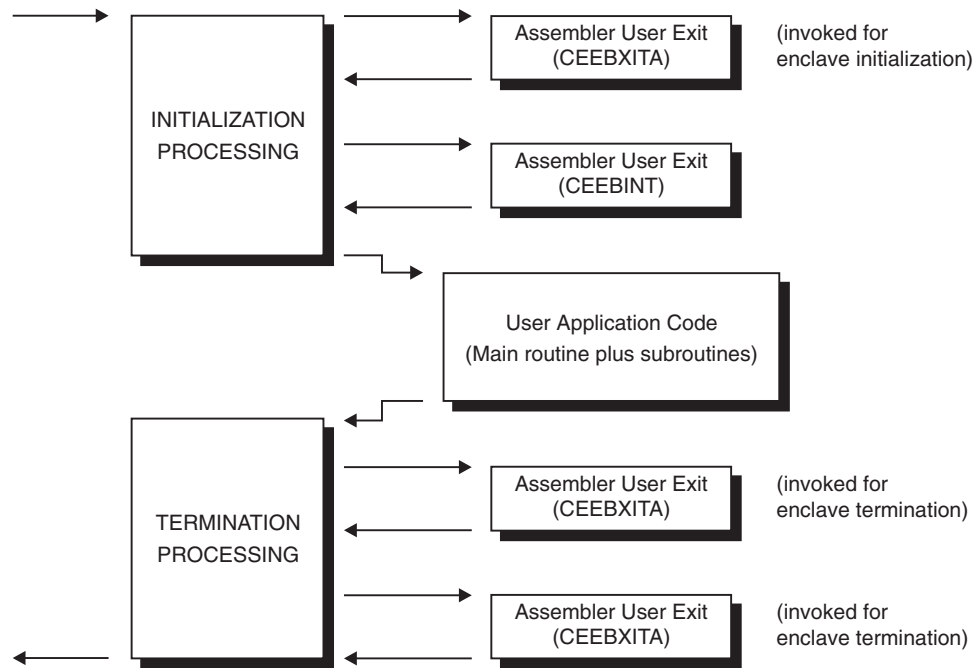
Figure 159. Location of User Exits
