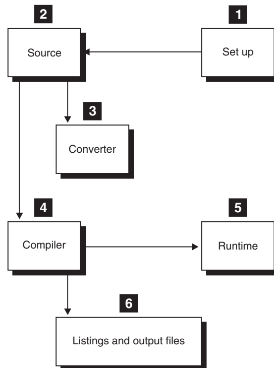
Figure 223. Compile-Edit, Related to Locale Function
