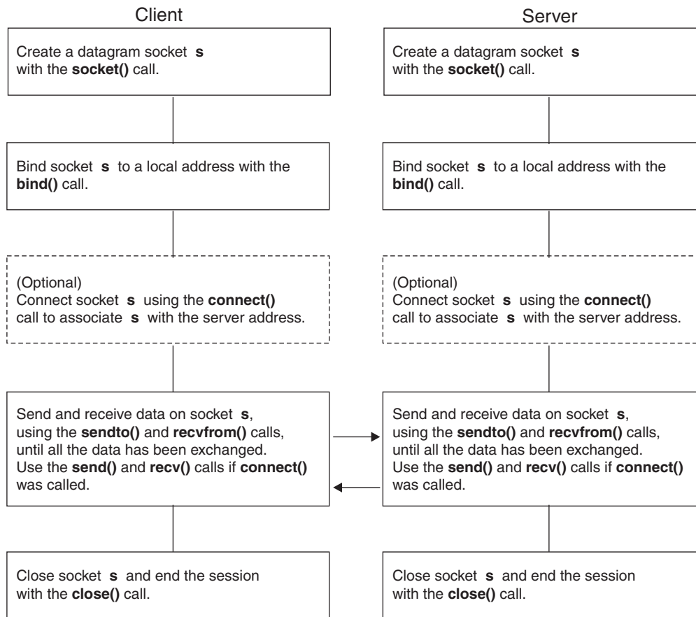
Figure 112. A Typical Datagram Socket Session
