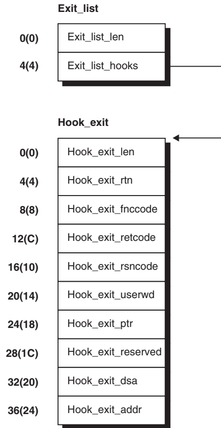
Figure 162. Exit_list and Hook_exit Control Blocks
