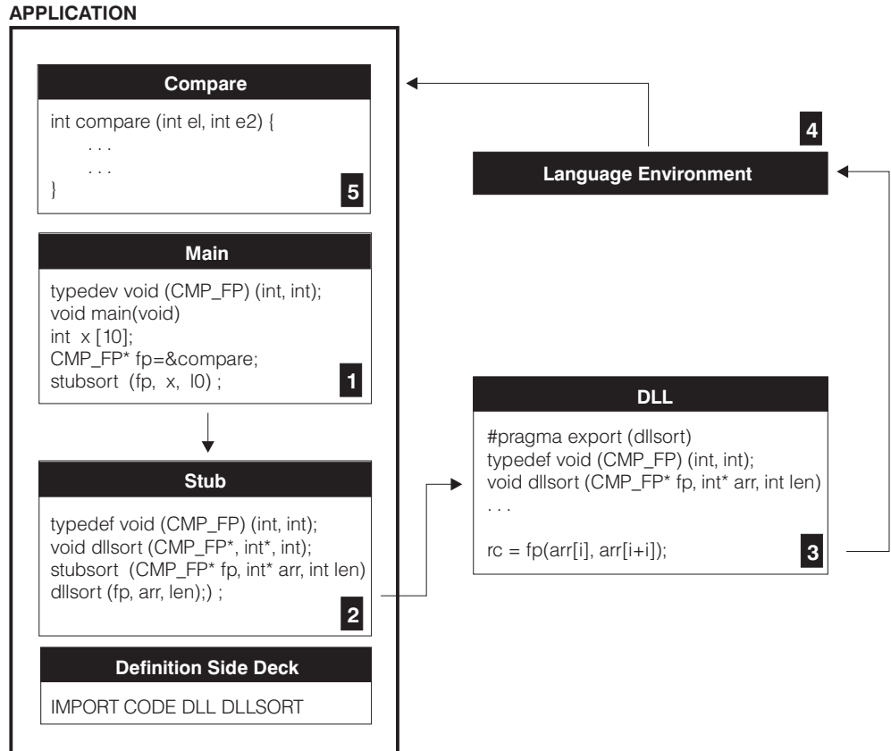
Figure 64. DLL Function Pointer Call in Non-Dll Code
