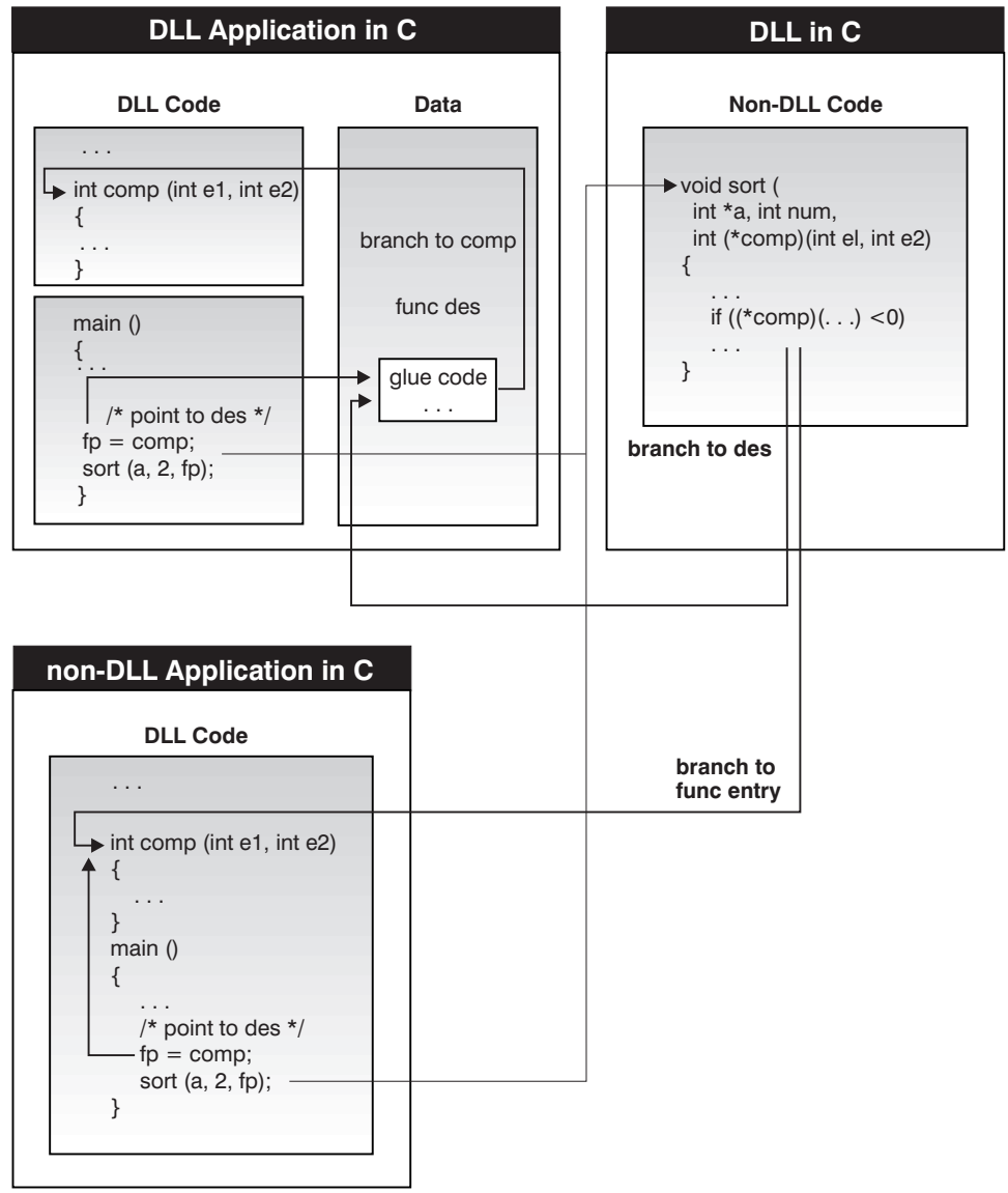
Figure 63. DLL Function Pointer Call in non-DLL code
