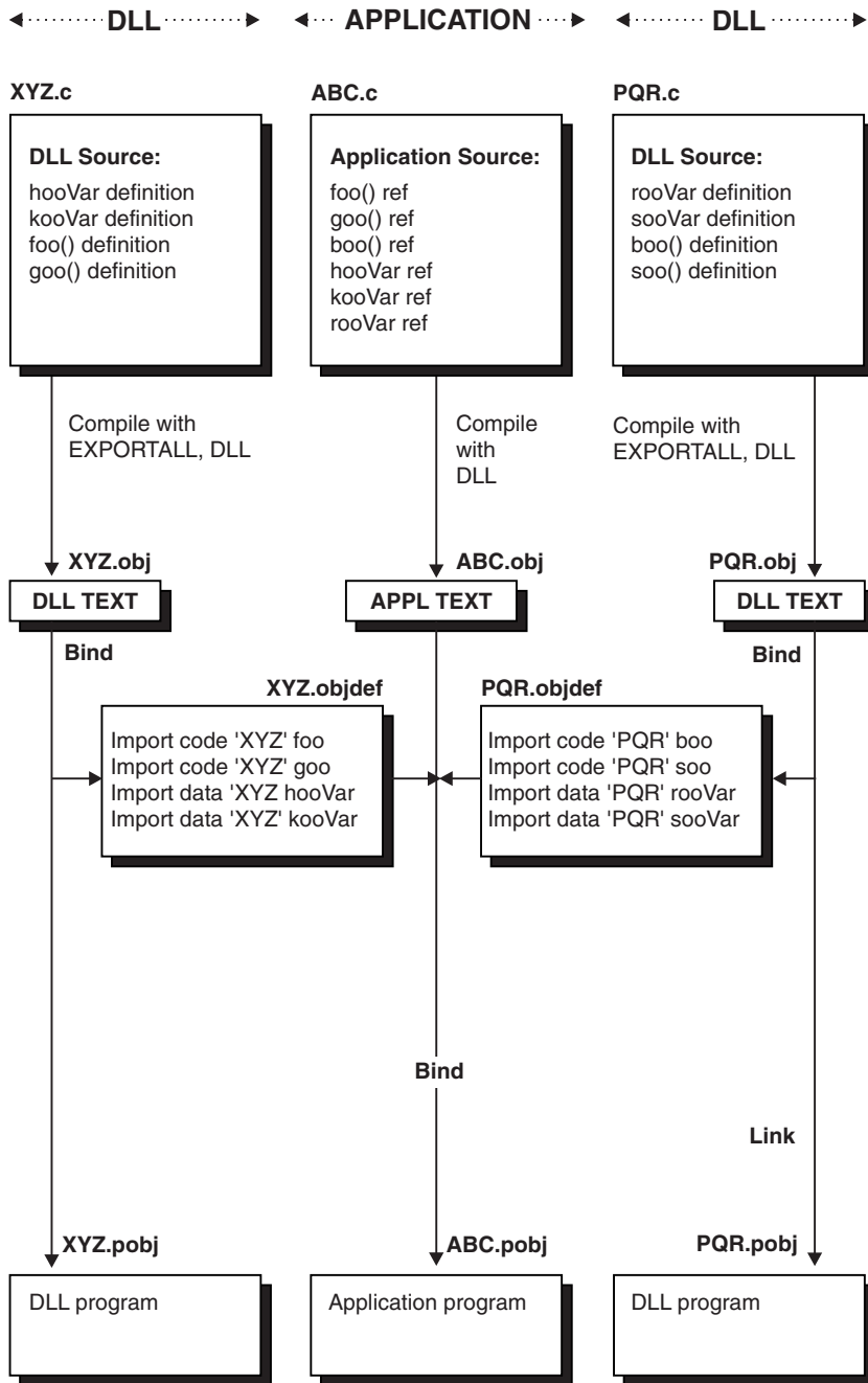
Figure 53. Summary of DLL and DLL Application Preparation and Usage
