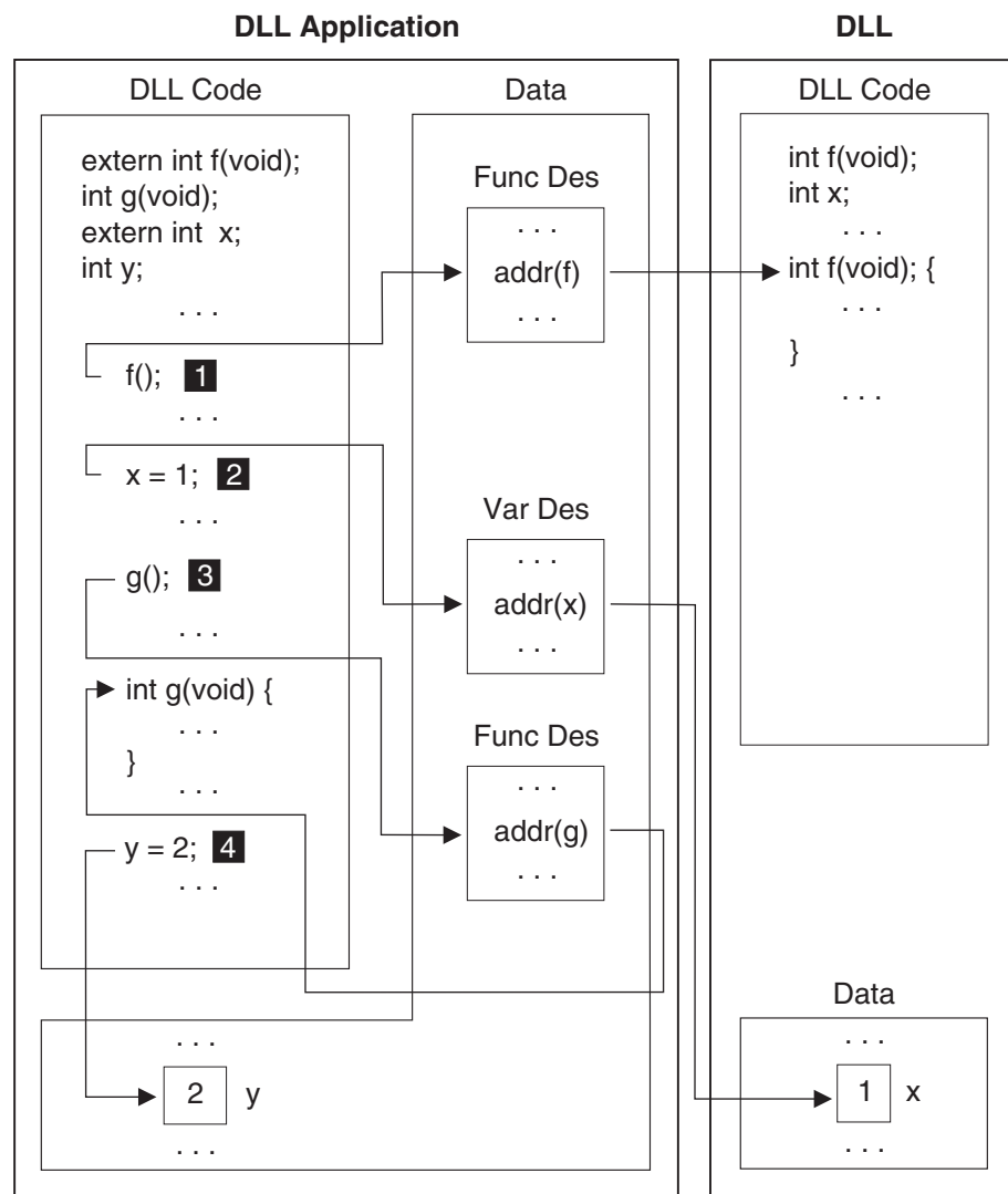
Figure 56. Referencing Functions and External Variables in DLL code
