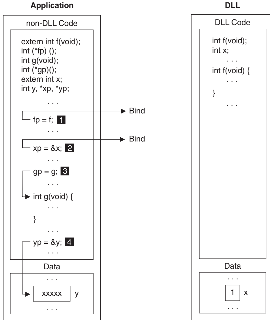
Figure 58. Pointer Assignment in Non-DLL code
