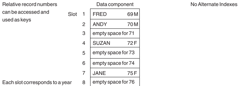
Figure 21. Types and Advantages of VSAM Data Sets
