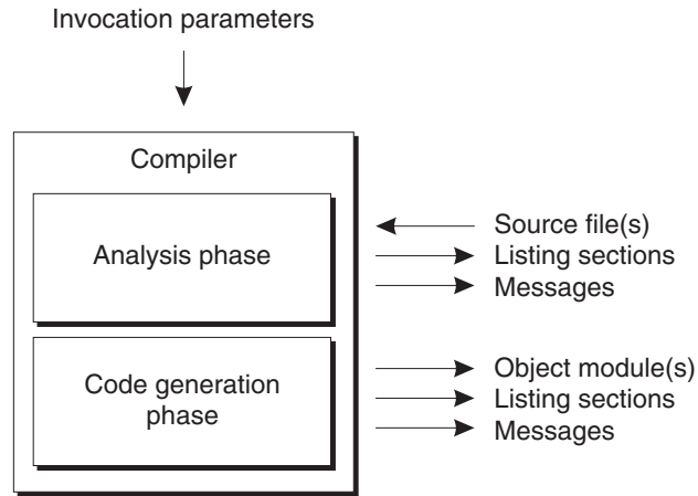
Figure 107. Flow of regular compiler processing
