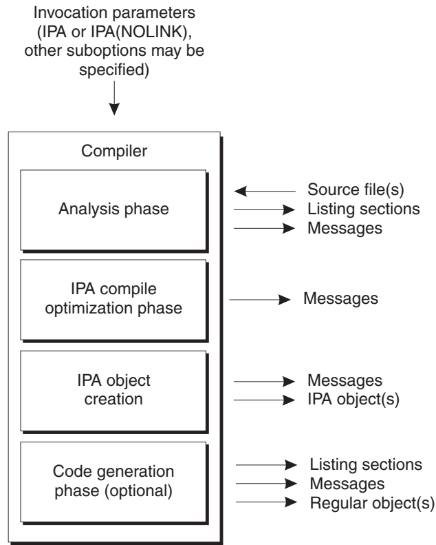
Figure 108. IPA Compile step processing
