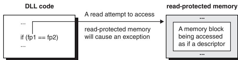
Figure 77. Comparison of Function Pointers in DLL code (C or C++)
