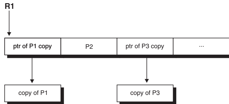
Figure 37. Example of Parameter Lists For OS Linkages
